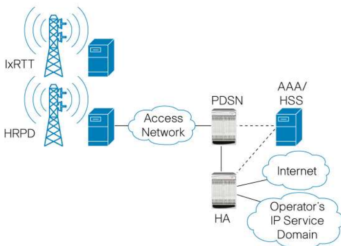
Figure 2. Example of Cisco UMTS Deployment.
