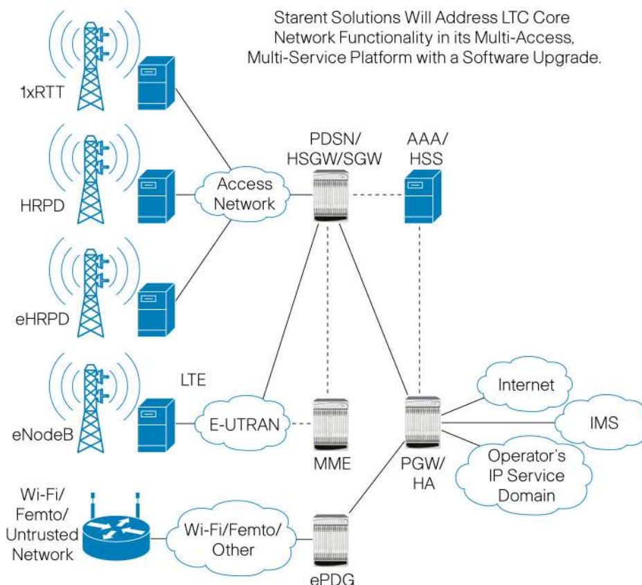
Figure 4. Addressing LTE Core Network Functionality in ASR 5000 with software upgrade
